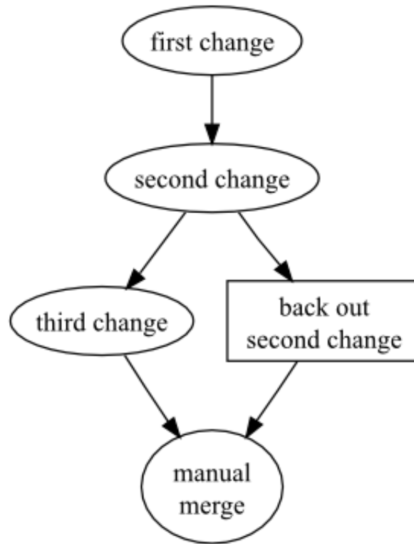
Figure 9.4: Manually merging a backout change
