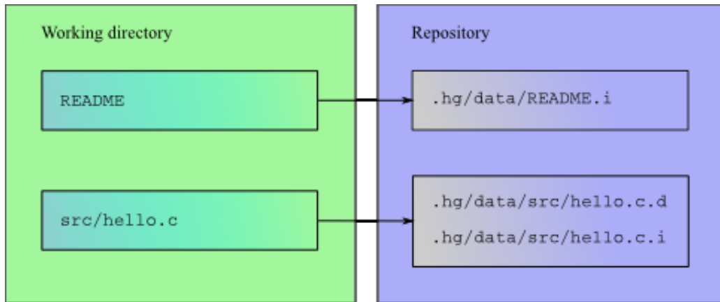
Figure 4.1: Relationships between files in working directory and filelogs in repository
